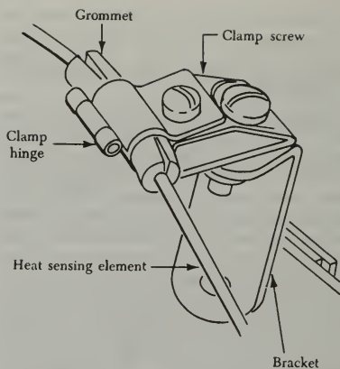
FIGURE 9-20. Typical fire detector loop clamp.
